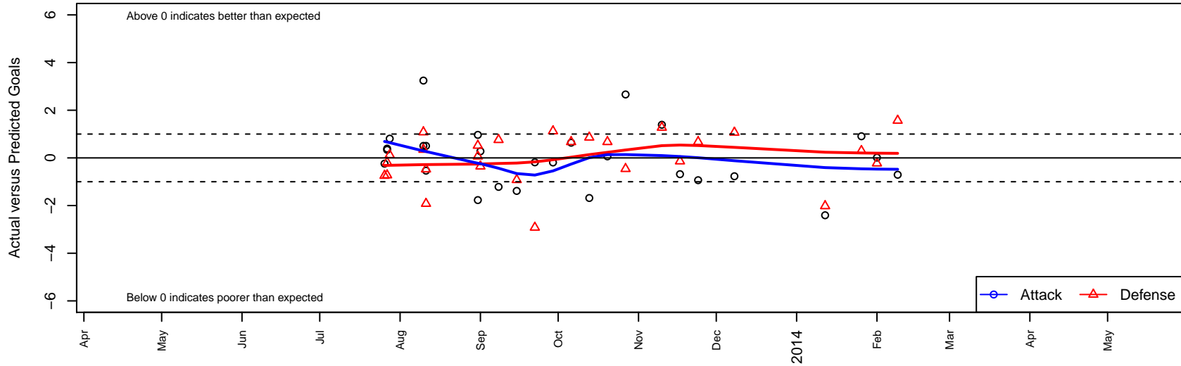
South Kitsap United B95 Dots are actual minus expected GF (blue circles) and GA (red triangles). Blue line is smoothed change in attack strength. Red is smoothed change in defense strength.
